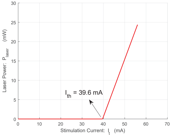
Fig. 6 Laser Power vs. Stimulation Current
